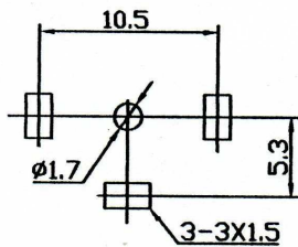
Dimensions of PC board holes(Commend)
